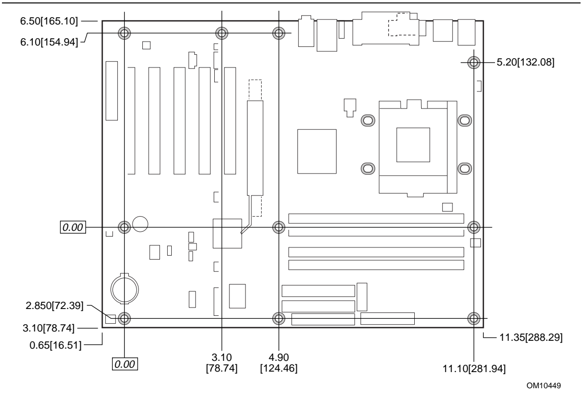
Figure 14. D850GB Board Dimensions
